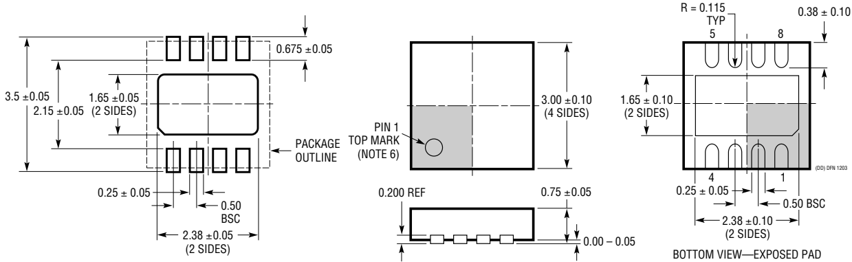
RECOMMENDED SOLDER PAD PITCH AND DIMENSIONS
