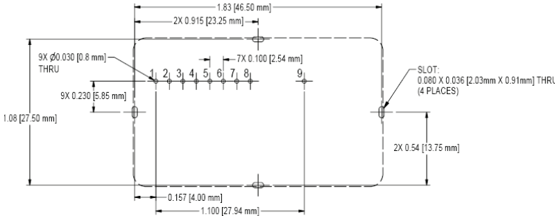
PCB MOUNTING (TOP VIEW)
