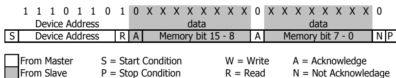
Figure 7: I 2 C answer from MS5805
