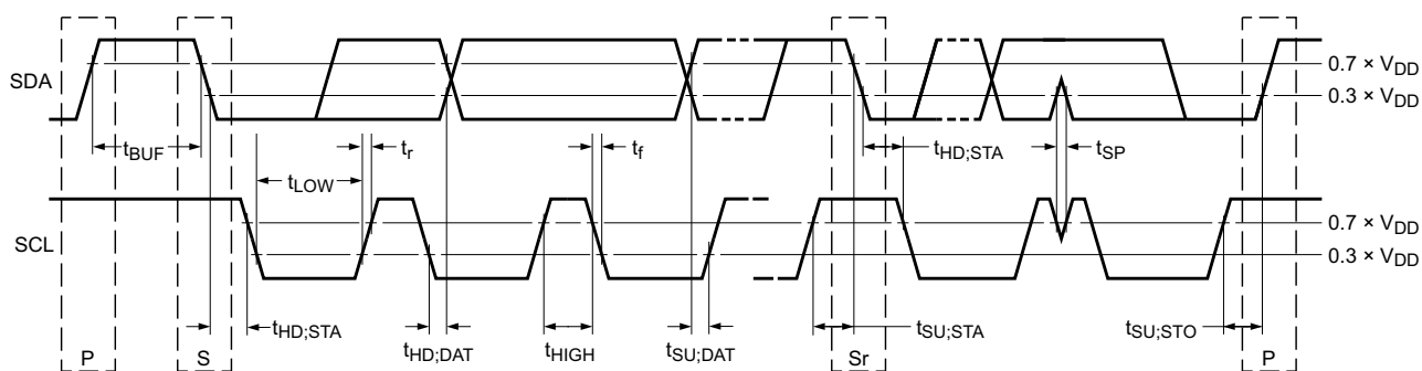
Fig 18. Definition of timing
