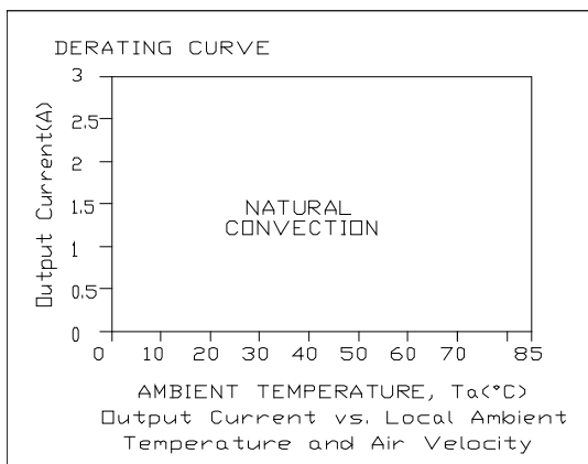
Figure 4. V_{in}=12\text{ V} , V_{out} = 1.2\text{ V}
