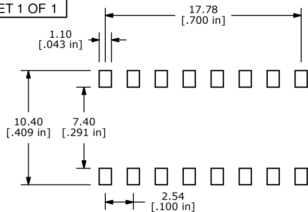
P.C.B. MOUNTING
