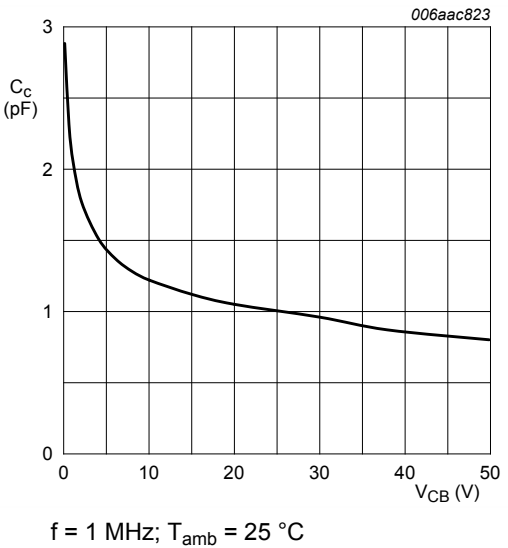
Fig. 9. NPN transistor: Collector capacitance as a function of collector-base voltage; typical values
