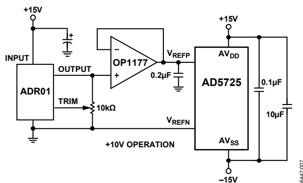
Figure 27. Unipolar +10 V Operation
