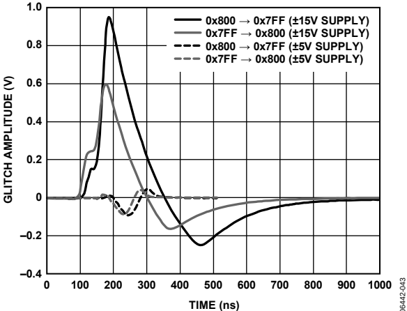
Figure 26. Output Glitch
