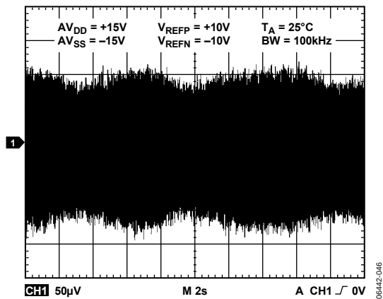
Figure 25. Broadband Noise
