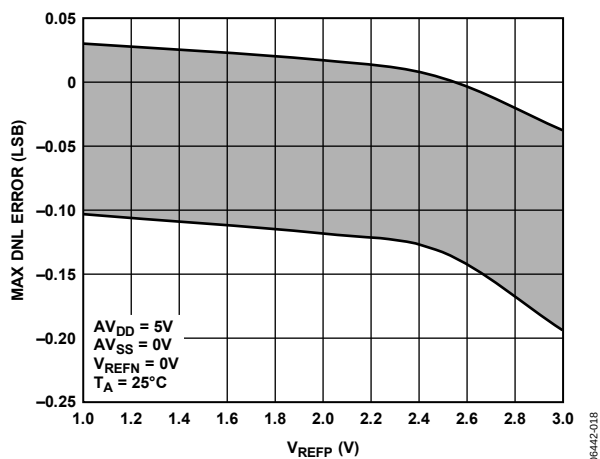
Figure 8. DNL vs. V_{REFP} ( V_{SUPPLY} = +5 V)
