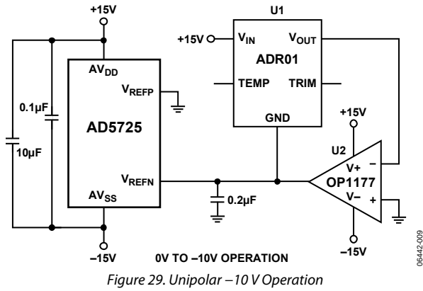
Figure 29. Unipolar -10\text{ V} Operation
