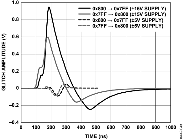
Figure 26. Output Glitch
