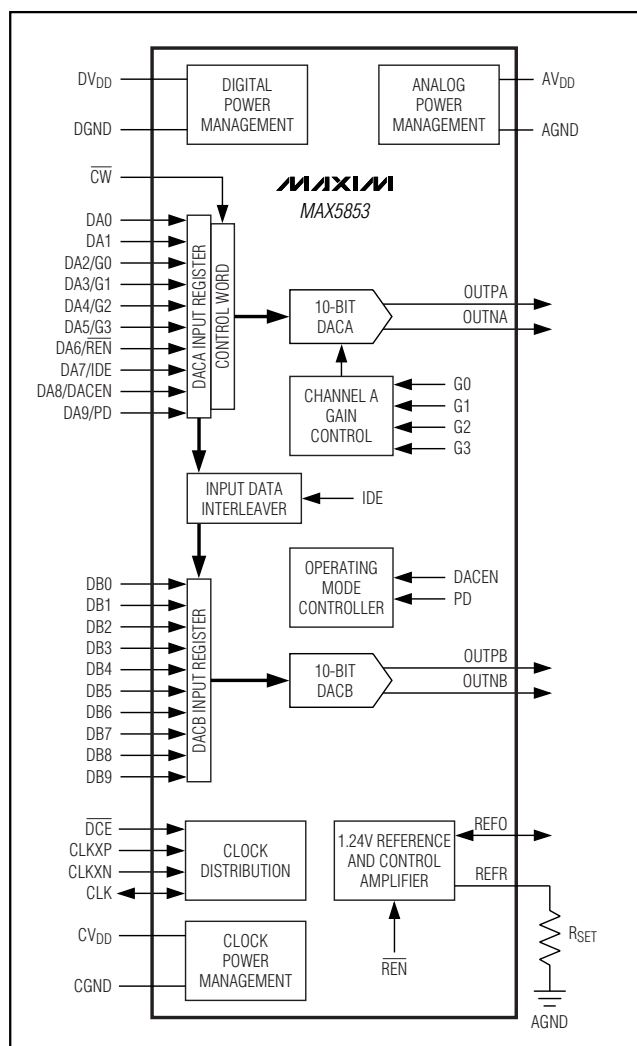
Figure 2. Simplified Diagram
