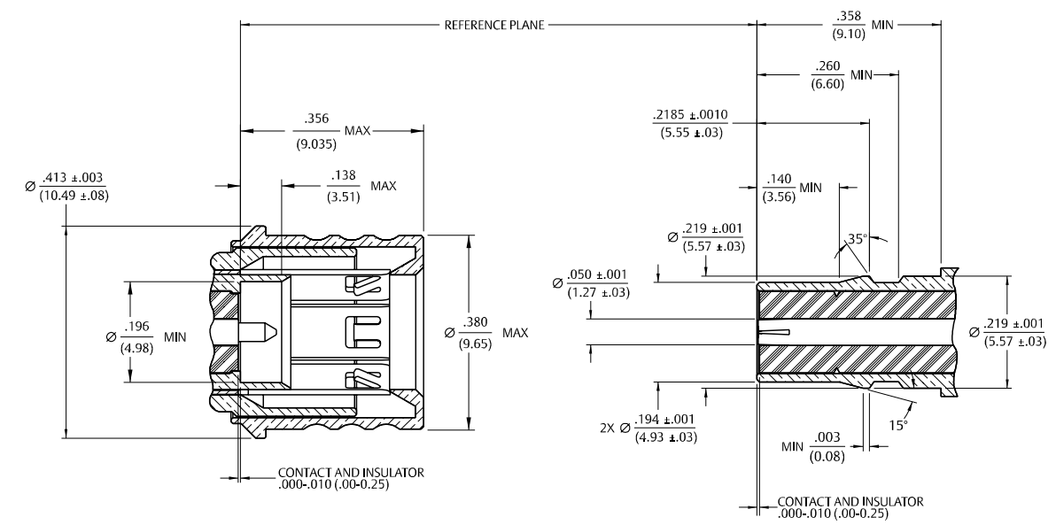
PLUG JACK
