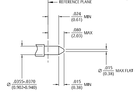
PLUG JACK
