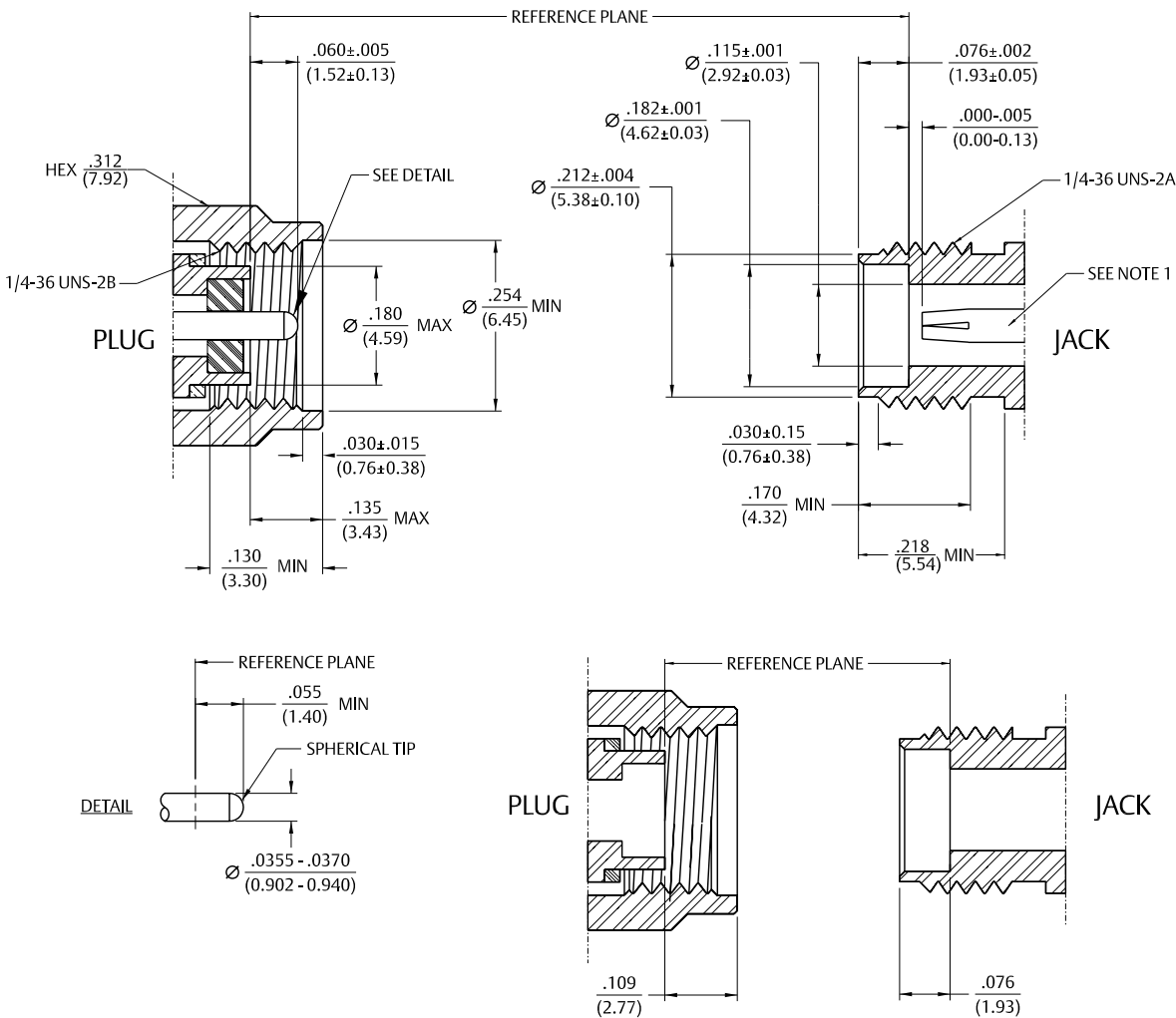
Mating Engagement for SMK (2.92mm) Series
