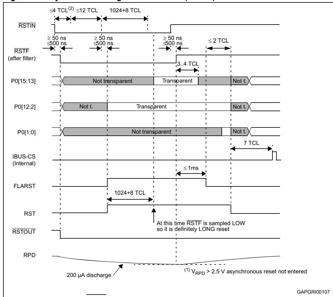
Figure 23. Synchronous long hardware reset ( \overline{\text{EA}} = 1 )
