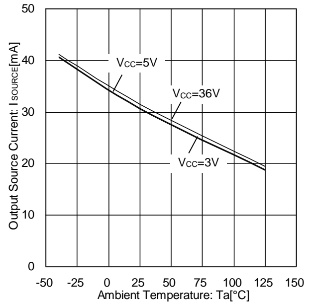
Figure 7. Output Source Current vs Ambient Temperature ( V_{OUT}=0V )
