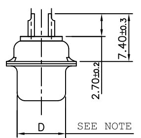
LAY OUT OF 50P CONNECTOR
