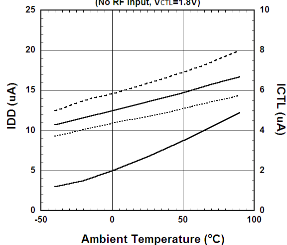
IDD, ICTL vs. Ambient Temperature
