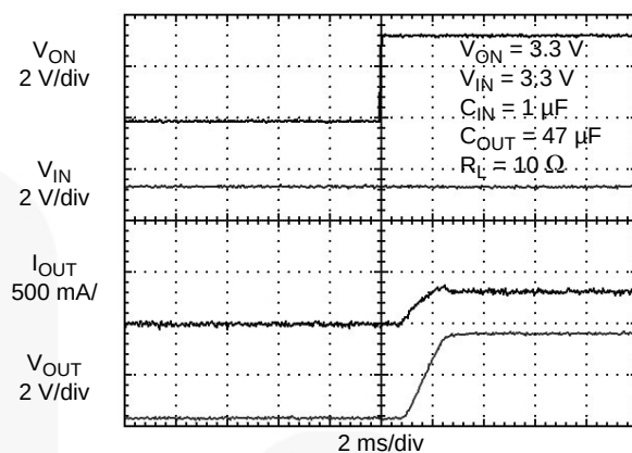
Figure 26. FPF1009 Turn-On Response ( C_{OUT} = 47 \mu\text{F} )
