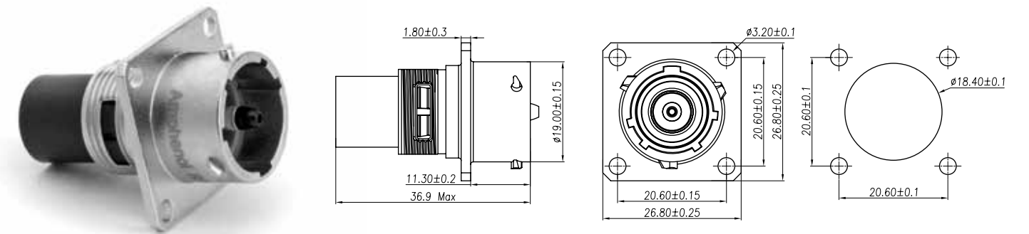
Wall Mounting Receptacle for Crimp Barrel
