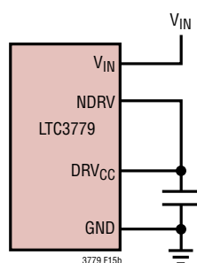
Figure 15b. Disabling the NDRV LDO
