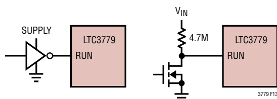
Figure 13. RUN Pin Interface to Logic
