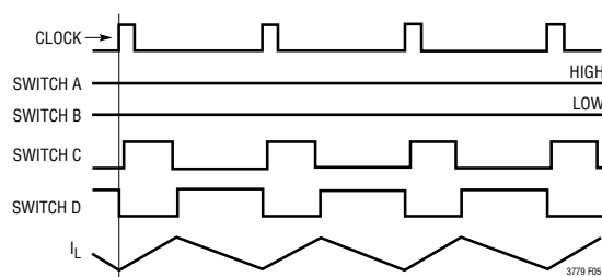
Figure 5. Boost Region ( V_{IN} \ll V_{OUT} )
