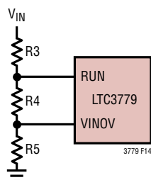
Figure 14. Adjustable UV and OV Lockout
