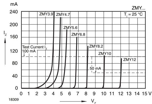
Fig. 6 - Breakdown Characteristics
