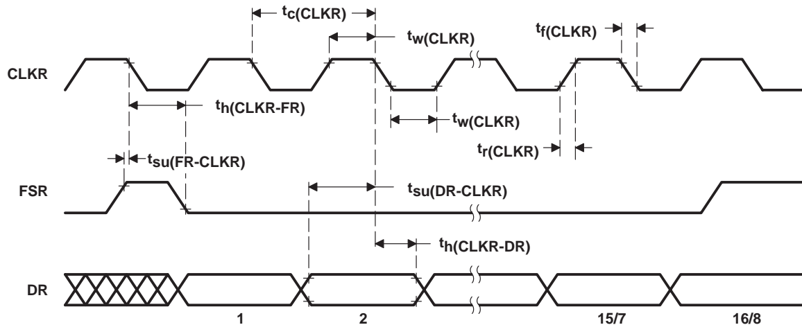
Figure 19. Serial-Port Receive Timing
