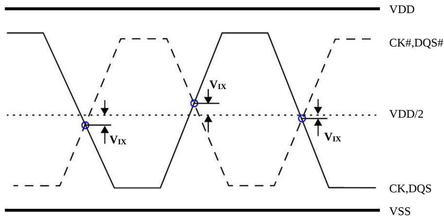
Figure 4.4. V_{IX} Definition
