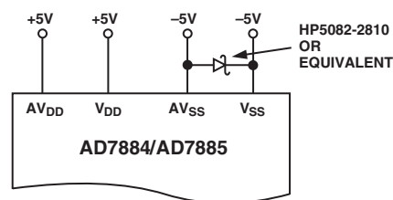
Figure 12. Schottky Diodes Used to Protect Against Incorrect Power Supply Sequencing
