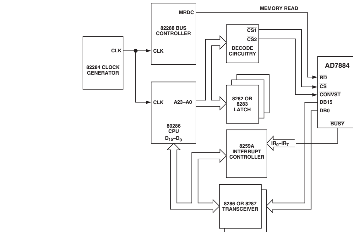
Figure 19. AD7884 Interfacing to Basic iAPX 286 System
