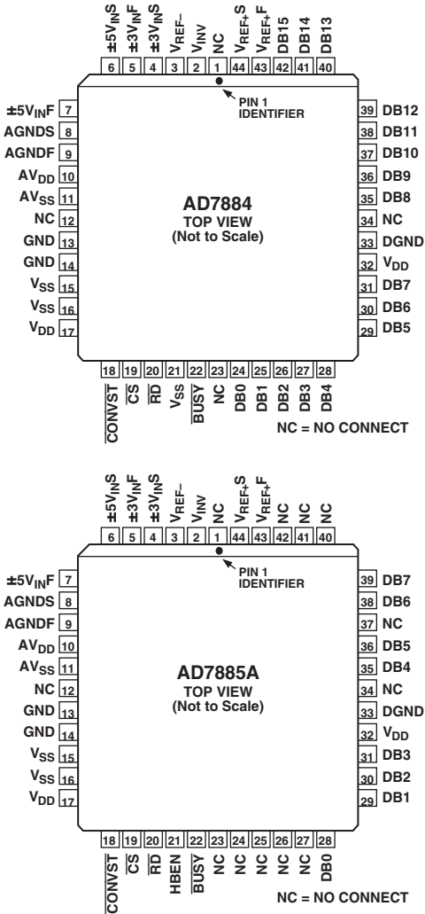
PLCC
