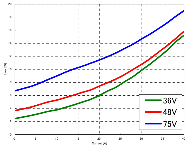
Fig-3: Power dissipation vs. load current and input voltage for converter mounted horizontally with airflow from pin 3 to pin 1 at a rate of 400LFM (2.0m/s) and Ta=25°C.
