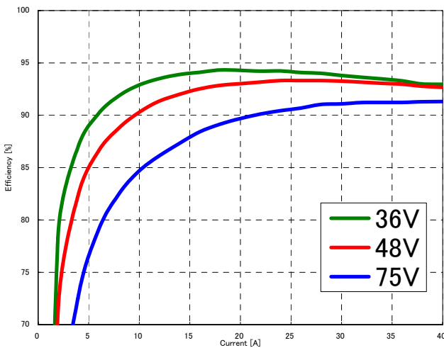
Fig-2: Efficiency vs. load current and input voltage for converter mounted horizontally with airflow from pin 3 to pin 1 at a rate of 400LFM (2.0m/s) and Ta=25°C.
