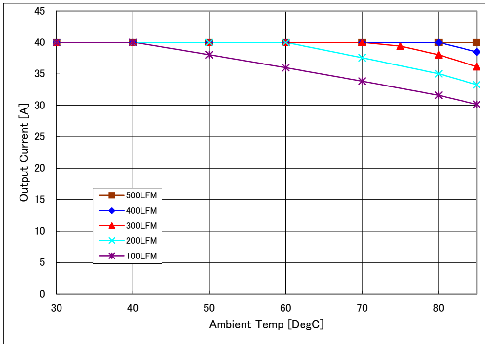
Fig-1: Available load current vs. ambient temperature and airflow rates for Vin=48V. Maximum component temperature \leq 125^{\circ}\text{C}
