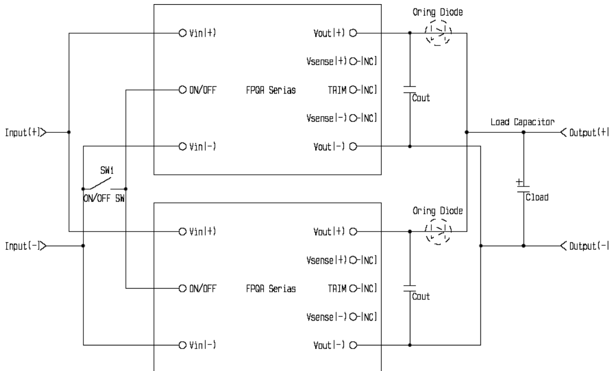
Sch-1 : Circuit for using the parallel option
