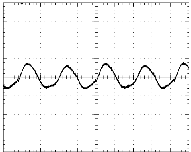
Fig-10: Input reflected ripple current, I_c (500mA/div), measured through 10 \mu H at the source at full rated load current and V_{in} =48V. Time scale: 1 \mu s/div.
