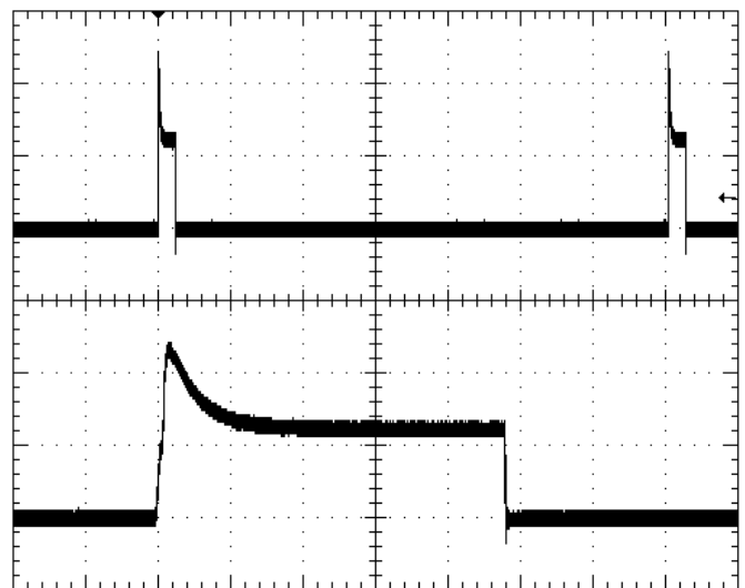
Fig-12: Load current (top trace, 50A/div, 40ms/div) into a 10m \Omega short circuit during restart, at V_{in} = 48V. Bottom trace (50A/div, 2ms/div) is an expansion of the top trace.
