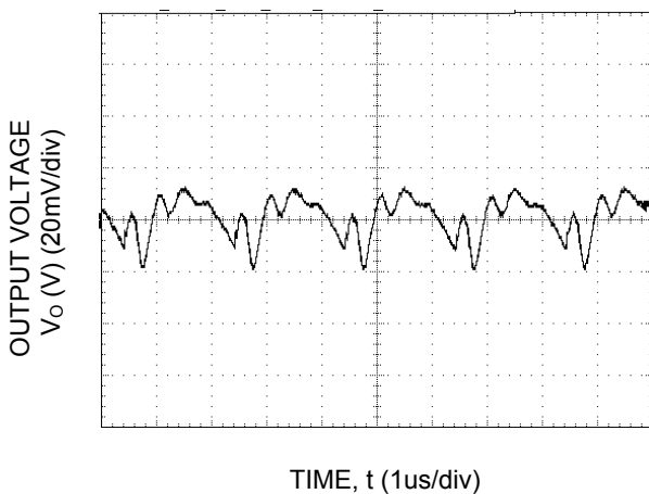
Fig-39. Typical output ripple and noise (CO=2x47µF ceramic, VIN = 12V, I o = I o,max , ).
