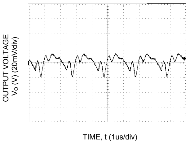
Fig-39. Typical output ripple and noise (CO=2x47uF ceramic, VIN = 12V, Io = Io,max, ).
