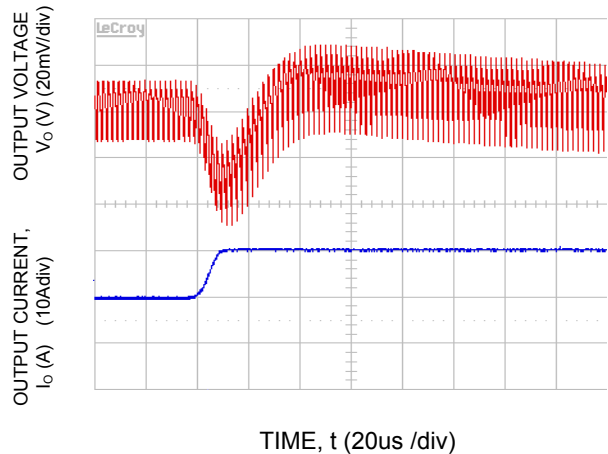
Fig-34. Transient Response to Dynamic Load Change from 50% to 100% at 12Vin, C out = 2x47μF +3x330μF, C Tune =5600pF & R Tune =220 ohms
