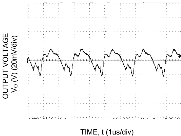
Fig-33. Typical output ripple and noise (C O =2X47μF ceramic, V IN = 12V, I o = I o,max ).
