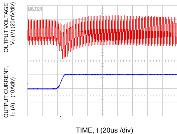
Fig-40. Transient Response to Dynamic Load Change from 50% to 100% at 12Vin, Cout= 1x47uF +5x330uF, CTune=10nF & RTune=178 ohms
