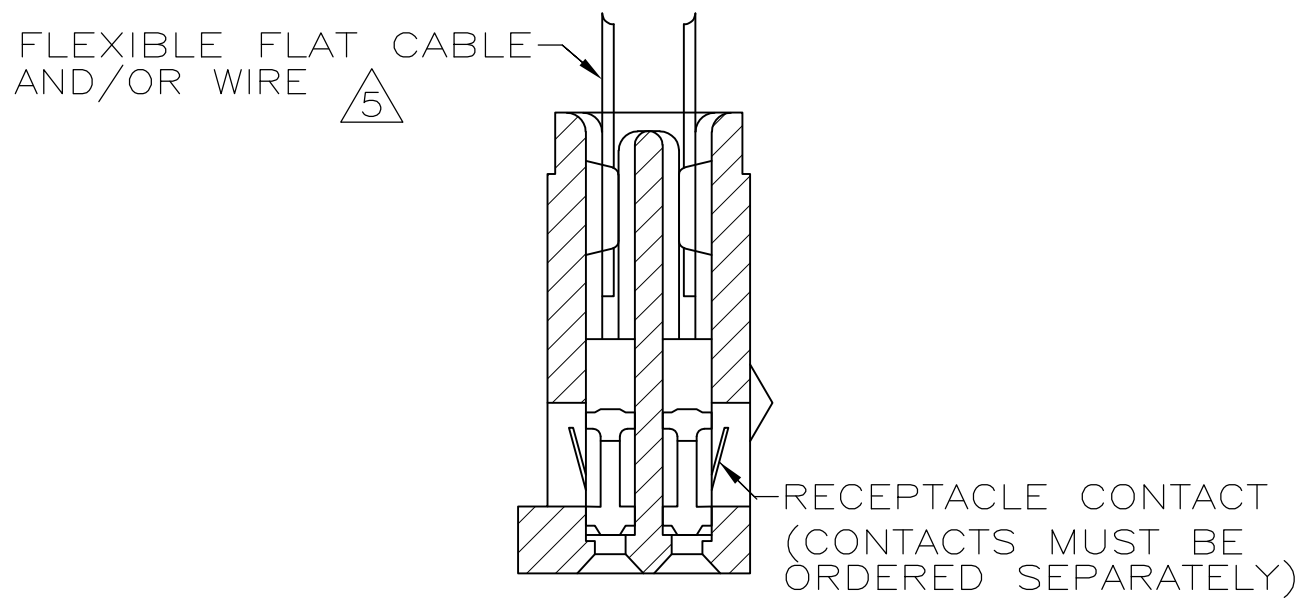
SECTION Y — Y LOADED HSG SCALE 4:1 (FOR REF ONLY)
