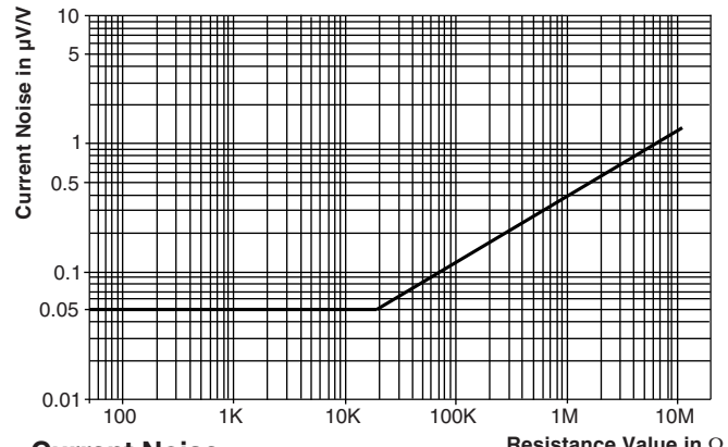
Current Noise
