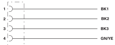
Contact assignment of the M12 socket
