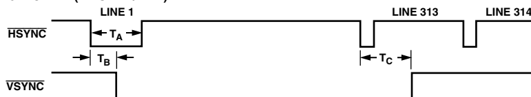
Figure 67. Timing Register 1
