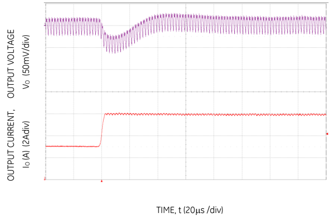
Figure 22. Transient Response to Dynamic Load Change on one output from 50% to 100% at 12Vin, Cout = 2x47µF + 1x330µF, CTune = 1500pF & RTune = 300Ω
