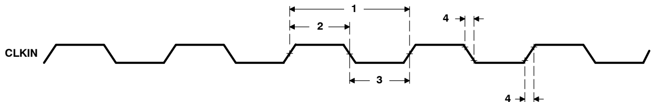
Figure 12. CLKIN Timings
