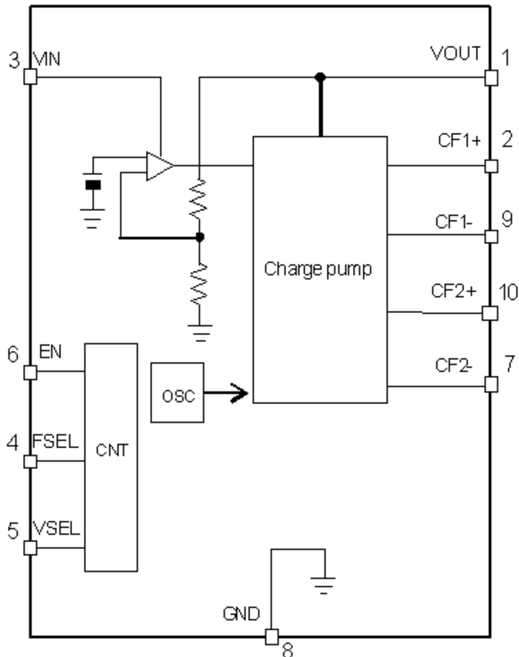
Figure 1. Block Diagram
