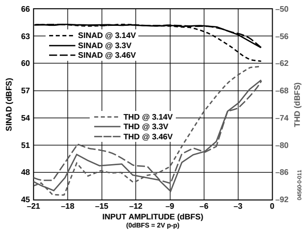
Figure 11. SINAD and THD vs. Input Amplitude and Supply ( f_{\text{IN}} = 8 \text{ MHz} , LPF f_{-3 \text{ dB}} = 26 \text{ MHz} ; R_{\text{xPGA}} = 0 \text{ dB} )
