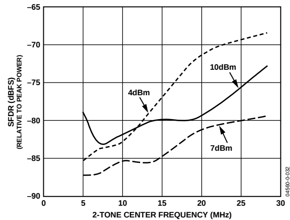
Figure 32. 2-Tone Worst Spur Frequency Sweep vs. Peak Power with f_{\text{DATA}} = 80 MSPS, 2 \times Interpolation
