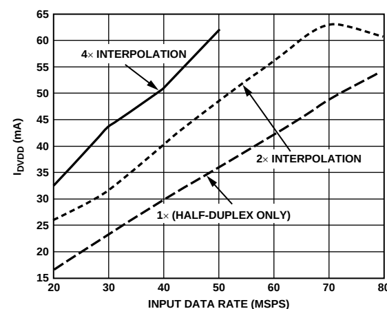
Figure 79. Digital Supply Current Consumption vs. Input Data Rate ( DVDD = DRVDD = 3.3 V and f_{OUT} = f_{DATA}/10 )
