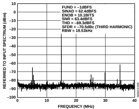
Figure 9. Spectral Plot with 4k FFT of Input Sinusoid with R_{\text{xPGA}} = 0 \text{ dB} and P_{\text{IN}} = 9 \text{ dBm}
