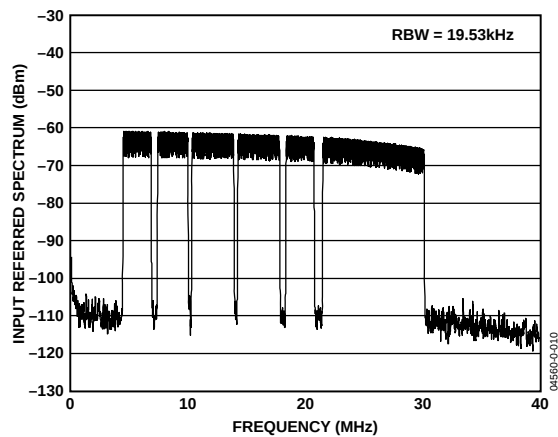
Figure 10. Spectral Plot with 4K FFT of 111-Carrier DMT Signal with \text{PAR} = 11 \text{ dB} , P_{\text{IN}} = -33.7 \text{ dBm} , LPF's f_{-3 \text{ dB}} = 32 \text{ MHz} and R_{\text{xPGA}} = 36 \text{ dB}
