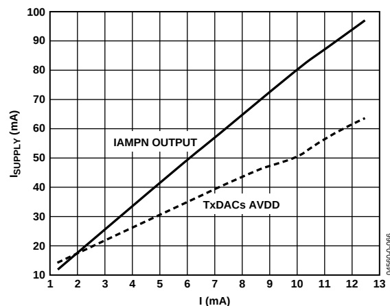
Figure 66. Current Consumption of TxDAC and IAMP in Current-Mode Operation with IOUTN Only (Default Settings)
