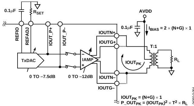
Figure 64. Current-Mode Operation
