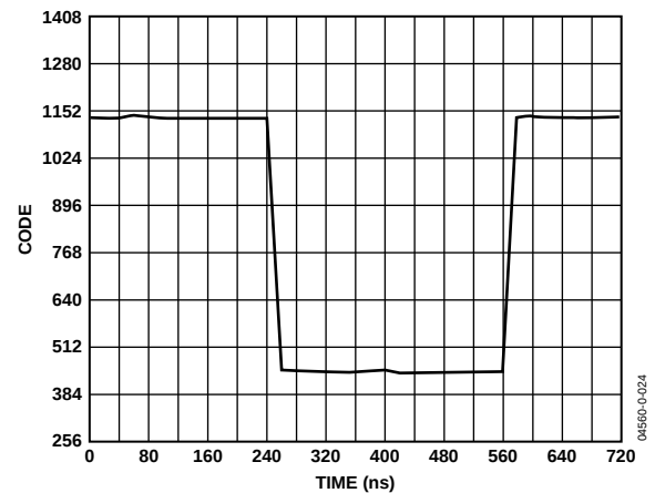
Figure 24. RxPGA Settling Time for 0 dB to +5 dB Transition for DC Input ( f_{\text{ADC}} = 50 MSPS, LPF Disabled)
