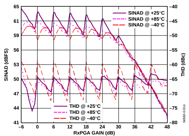
Figure 14. SINAD/THD Performance vs. R_{\text{xPGA}} Gain and Temperature ( f_{\text{IN}} = 10 \text{ MHz} )
