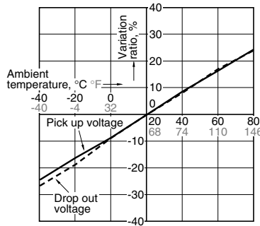
1.-(2) Ambient temperature characteristics (20A type)
