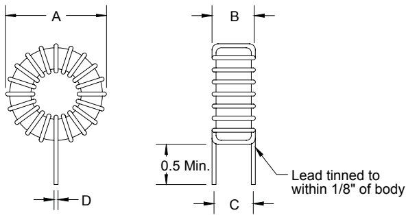
Dimensions: Inches
