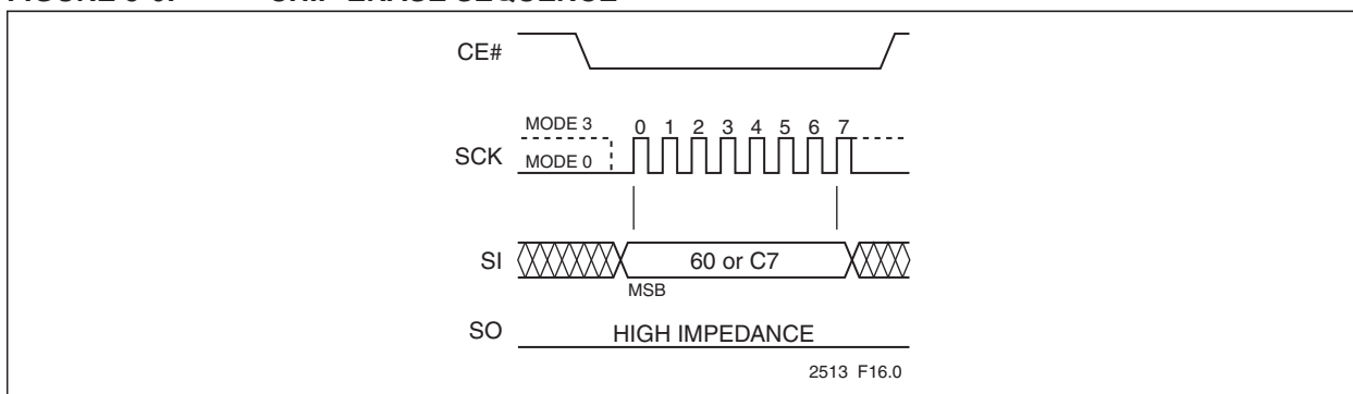
FIGURE 5-6: CHIP-ERASE SEQUENCE
