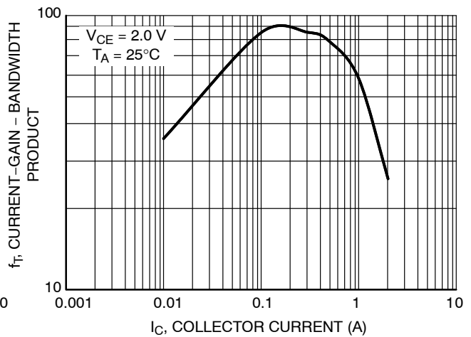
Figure 6. Current-Gain-Bandwidth Product
