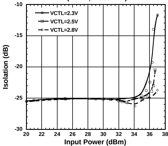
Isolation vs. Input Power (P1-P2, f=1.9\text{GHz} )
