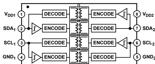
Figure 1. ADuM1250
