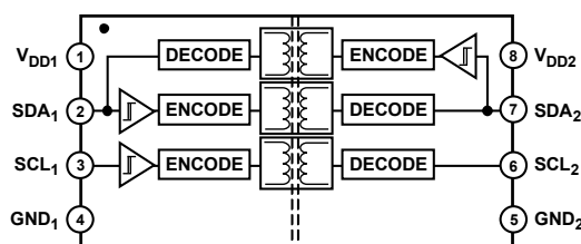
Figure 2. ADuM1251
