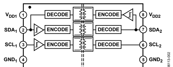
Figure 2. ADuM1251
