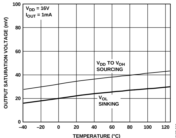
Figure 12. Output Saturation Voltage vs. Temperature
