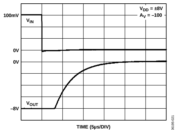
Figure 23. Negative Overload Recovery Time
