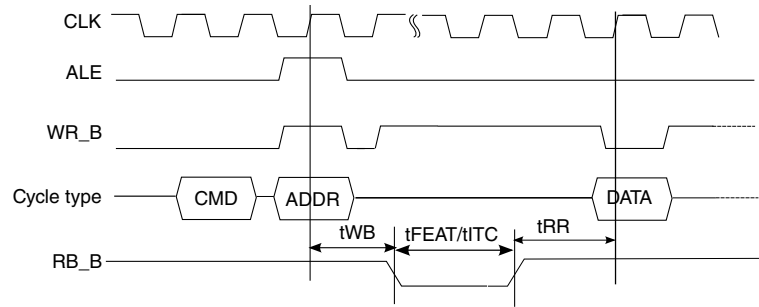
Figure 59. t_{WB} , t_{FEAT} , t_{ITC} , and t_{RR} timings
