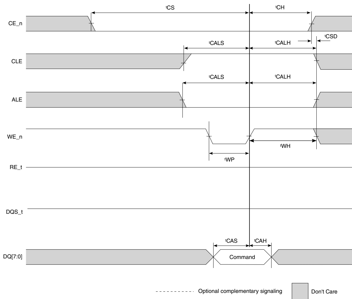
Figure 55. Command cycle
