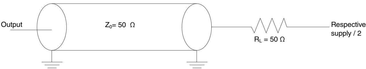
Figure 47. Integrated Flash Controller AC test load
