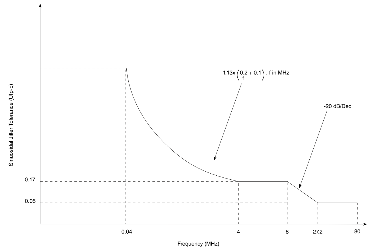
Figure 44. XFI host receiver input sinusoidal jitter tolerance
