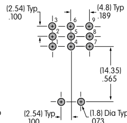
Three Pole
