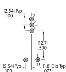
Single Pole
