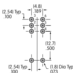
Double Pole
