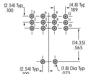
Four Pole
