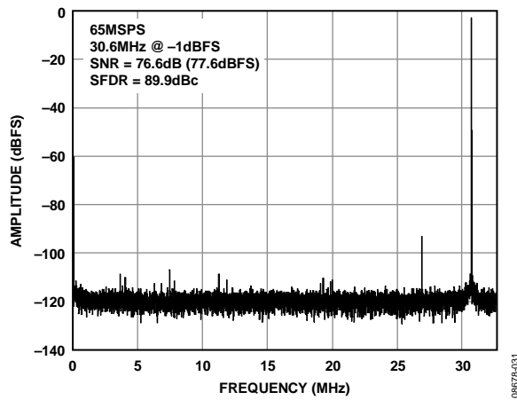
Figure 18. AD9266-65 Single-Tone FFT with f_{IN} = 30.6 MHz
