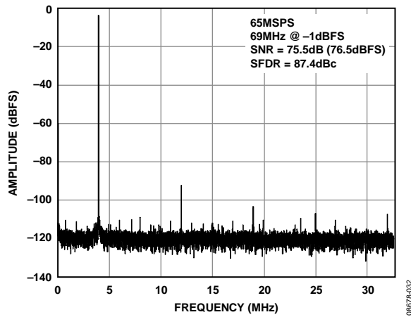
Figure 17. AD9266-65 Single-Tone FFT with f_{IN} = 69 MHz
