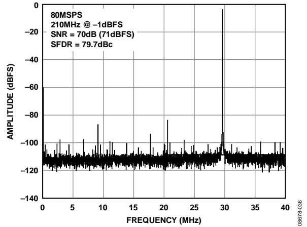
Figure 8. AD9266-80 Single-Tone FFT with f_{IN} = 210 MHz
