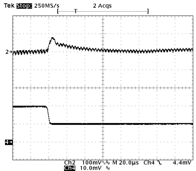
Fig-1.5V-7: Output voltage response for Vout=1.5V to negative load current step change from 10A to 5A with slew rate of -5A/us at Vin=12V. Co=47uFx2 ceramic. Top trace: output voltage (100mV/div.) Bottom trace: load current (5A/div.) Time scale: 20us/div.
