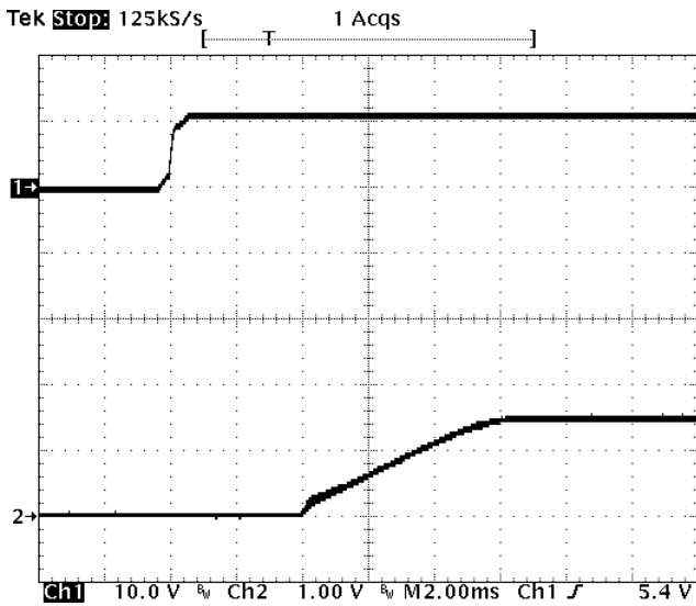
Fig-1.5V-4: Turn-on transient for Vout=1.5V with application of Vin at full rated load current (resistive) and 47uFx2 external capacitance at Vin=12V. Top trace: Vin (10V/div.) Bottom trace: output voltage (1V/div.) Time scale: 2 ms/div.
