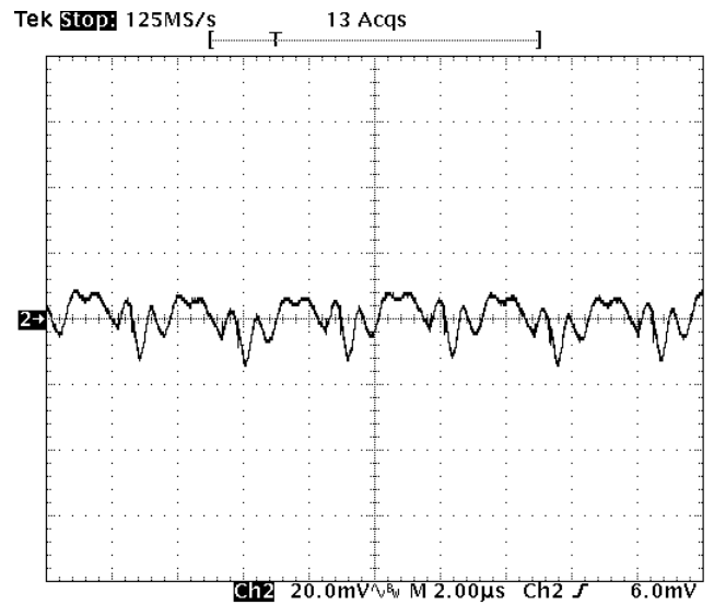
Fig-1.5V-5: Output voltage ripple (20mV/div.) for Vout=1.5V at full rated load current into a resistive load with external capacitance 47uFx2 ceramic + 1uF ceramic at Vin=12V. Time scale: 2us/div
