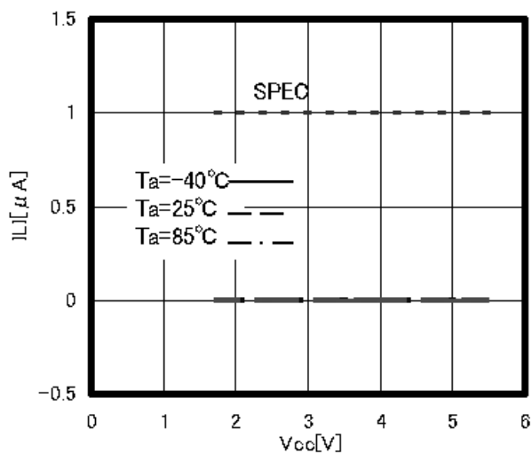
Figure 8. Input Leak Current I_{LI} (CSB, SCK, SI, HOLDB, WP)
