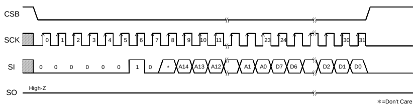
Figure 34. Write command
