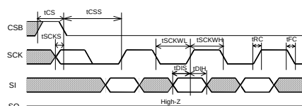
Figure 1. Input timing
