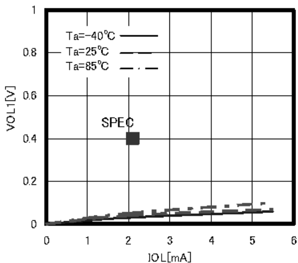
Figure 6. "L" Output Voltage V_{OL} ( V_{CC} = 2.5\text{V} )
