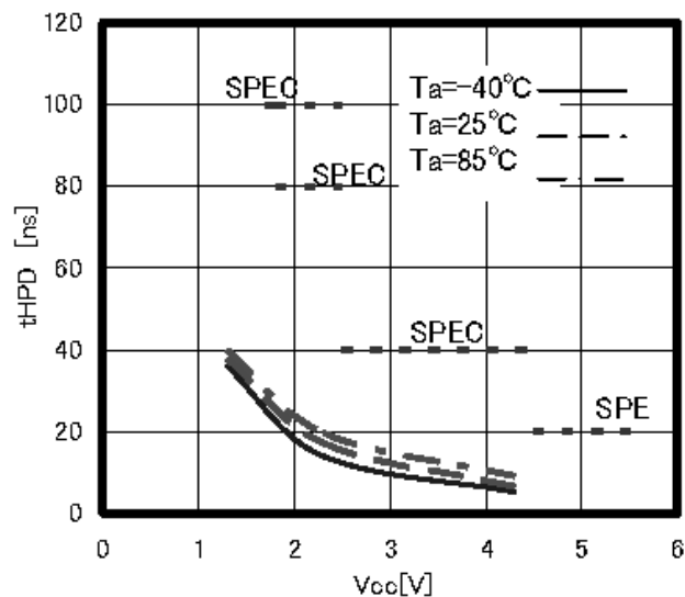
Figure 27. Time from HOLD to output change tHPD
