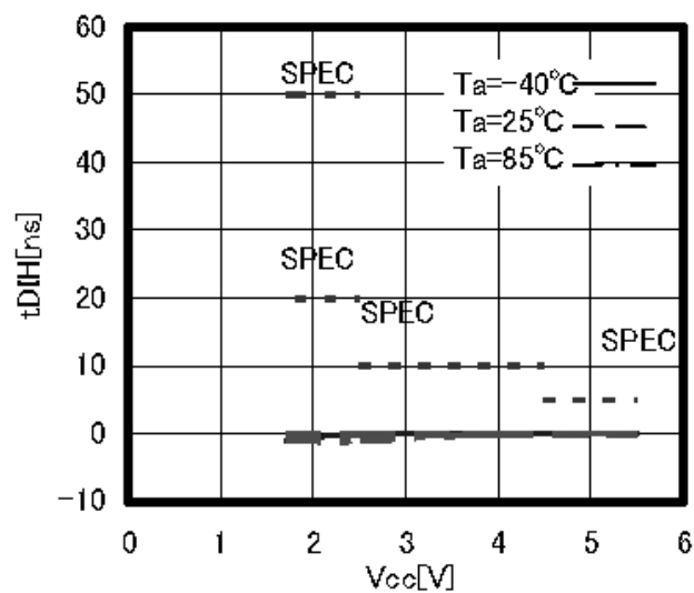
Figure 21. SI hold time t_{DIH}
