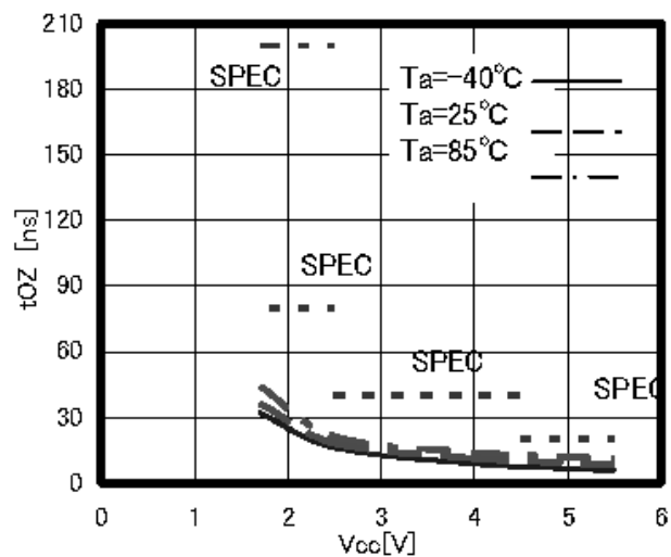
Figure 23. Output disable time t_{OZ}
