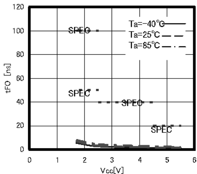
Figure 29. Output fall time t_{FO}
