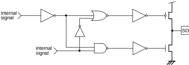
Figure 46. SO output equivalent circuit
