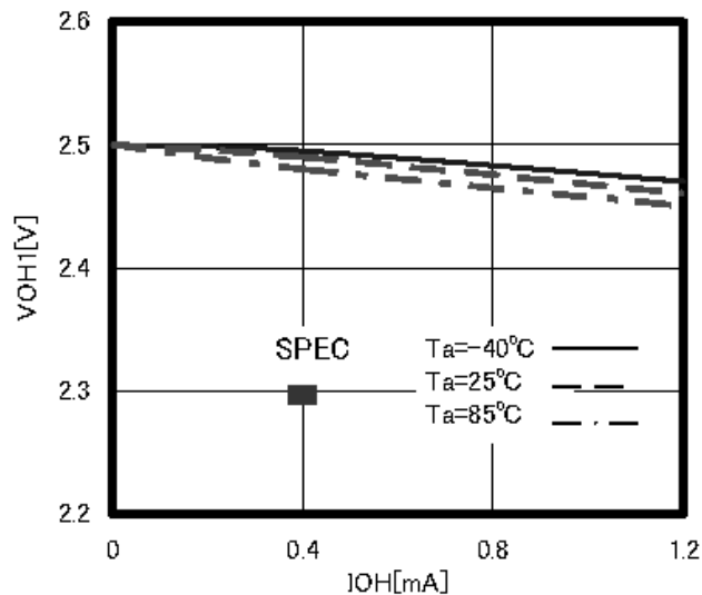
Figure 7. "H" Output Voltage V_{OH} ( V_{CC} = 2.5\text{V} )
