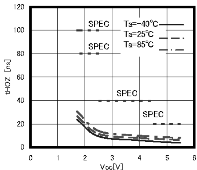
Figure 26. Time from HOLD to output High-Z tHOZ
