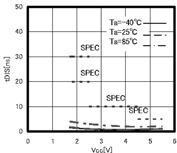
Figure 20. SI setup time t_{DIS}
