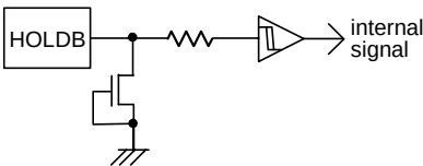
Figure 50. HOLDB input equivalent circuit
