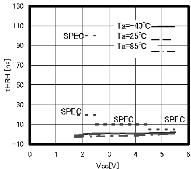
Figure 25. HOLD release hold time tHRH
