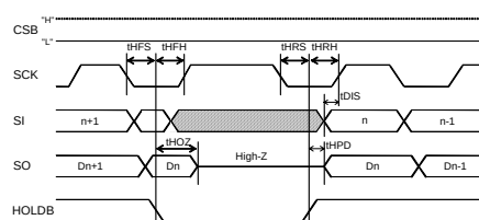
Figure 3. HOLD timing
