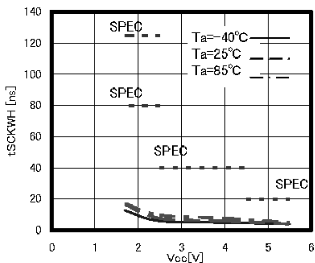
Figure 15. SCK high time tSCKWH
