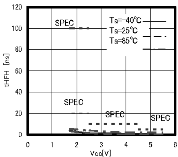
Figure 24. HOLD setting hold time tHFH
