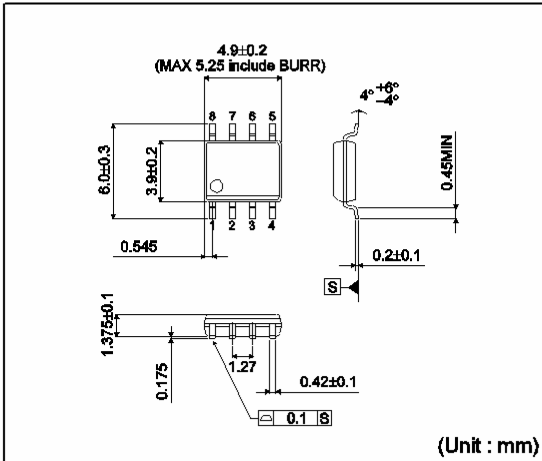
SOP-J8
