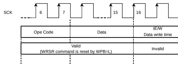
Figure 37. \overline{\text{WP}} valid timing (At inputting WRSR command)
