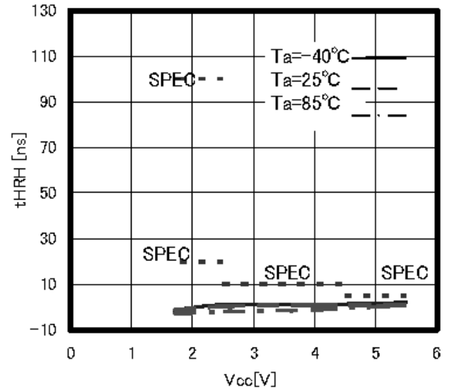
Figure 25. HOLD release hold time tHRH
