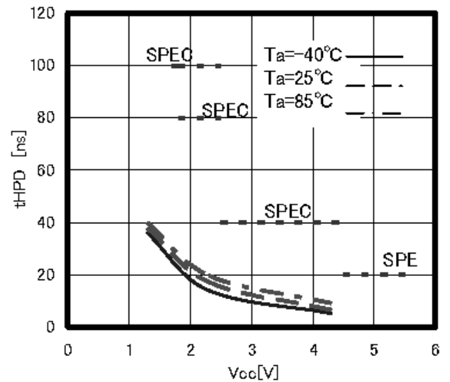
Figure 27. Time from HOLD to output change tHPD
