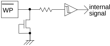
Figure 51. WP input equivalent circuit
